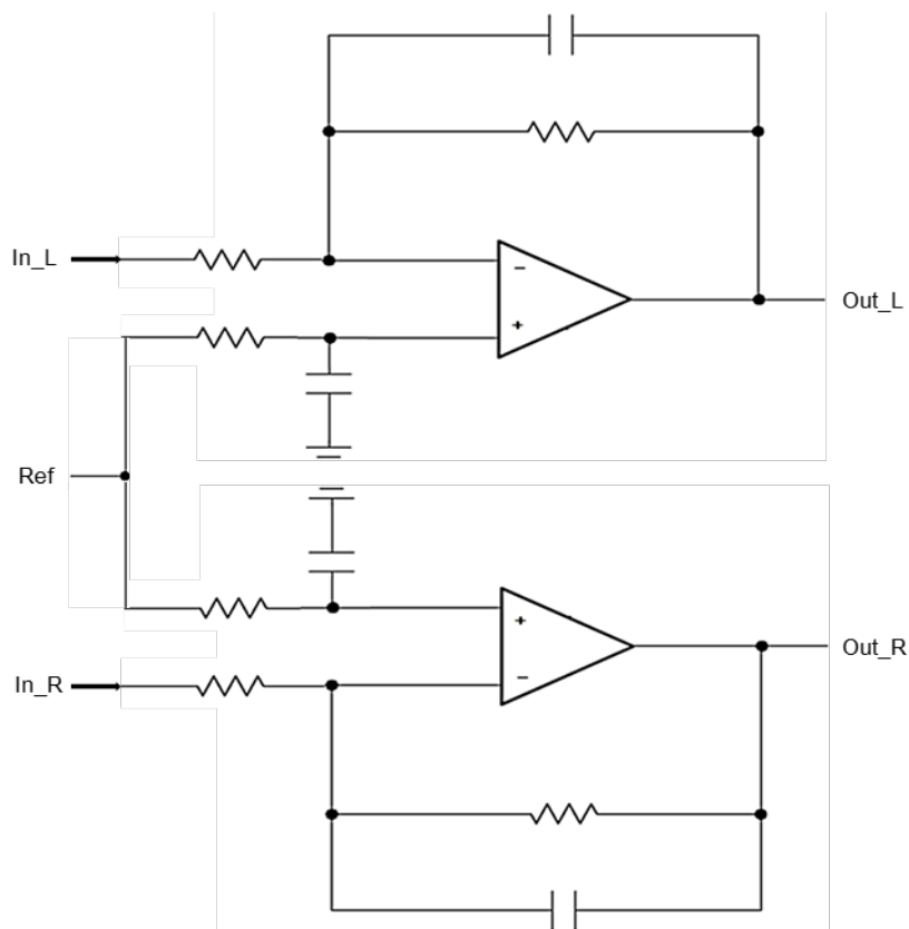
ication Circuit (Stereo Sound Input Amplifier)
