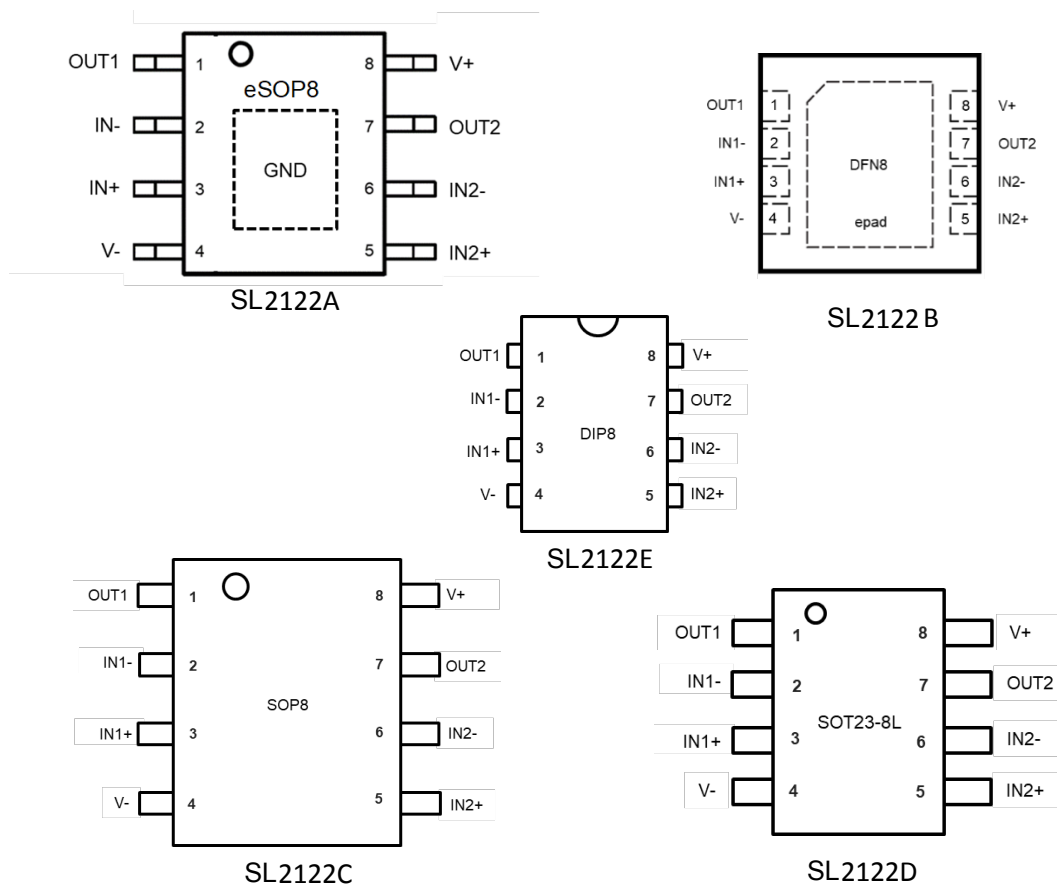
Figure 3 SL2122A/B/C/D/E Pinouts
