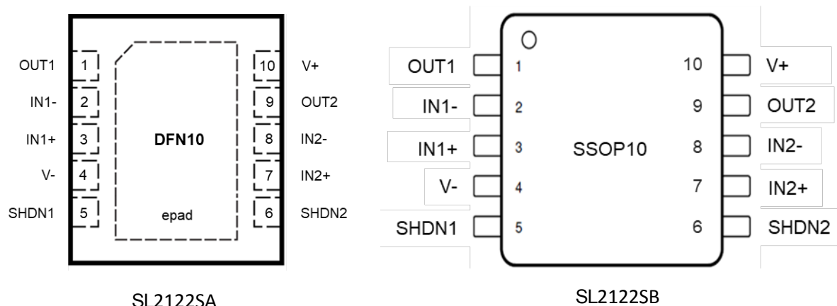
Figure 4 SL2122SA/B Pinouts
